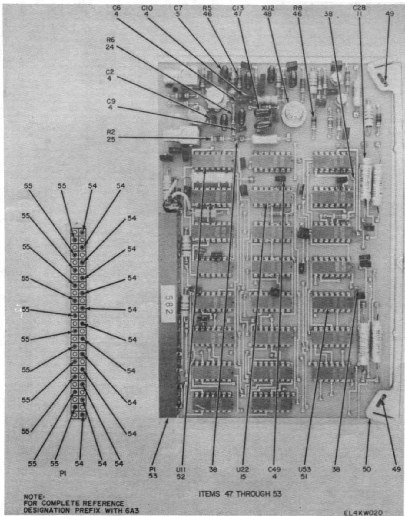
Figure 10. Mixer/Variable Divider Card 6A3 (Sheet 3 of 3).
