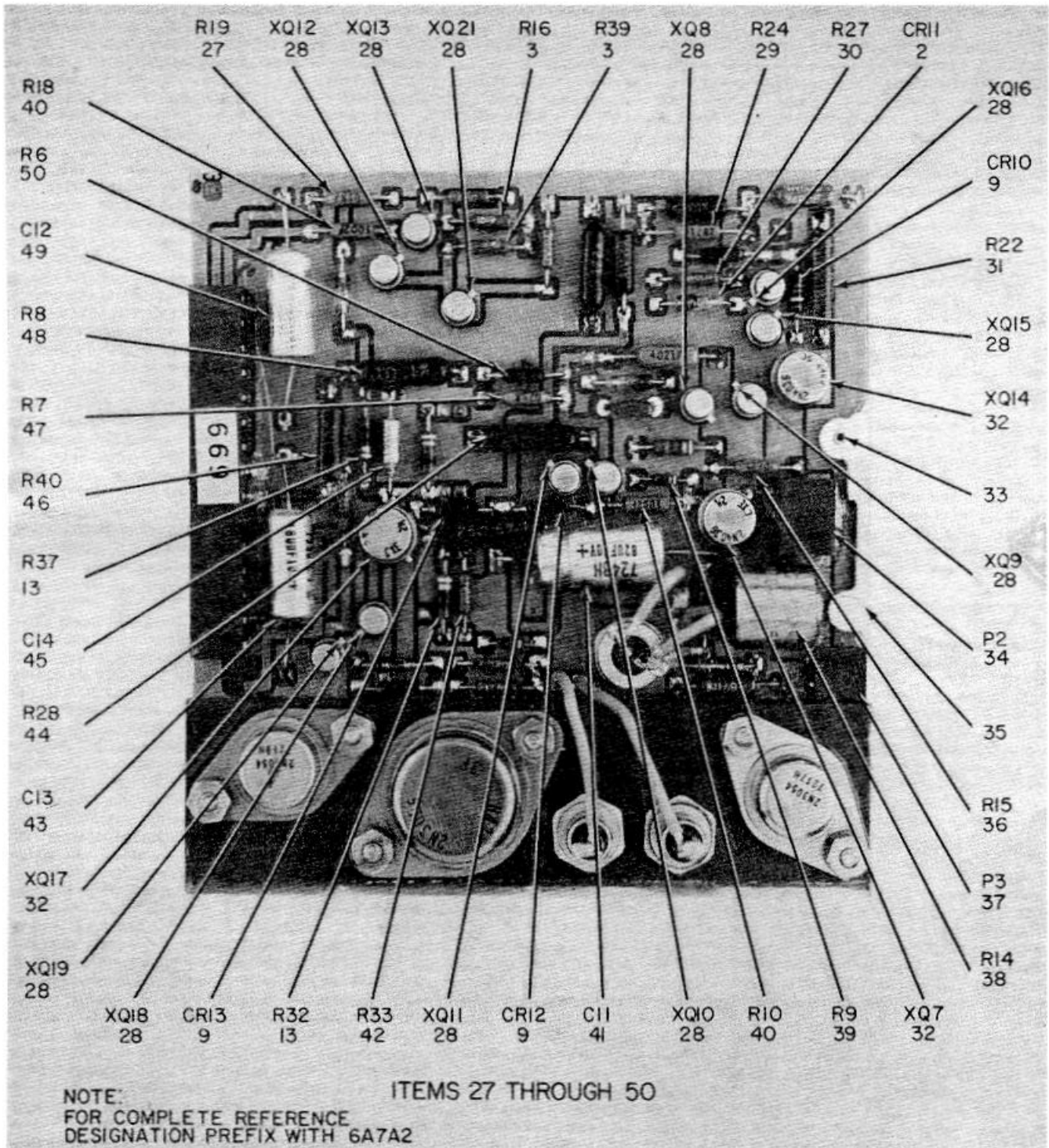
Figure 18. Regulator Card 6A7A2 (Sheet 2 of 4).
