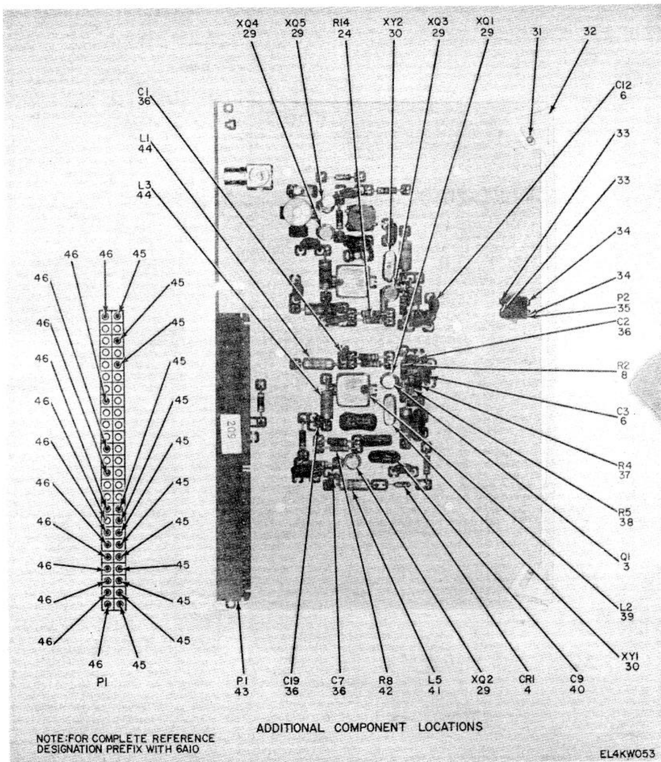
Figure 21. Injection Oscillator Card 6A10 (Sheet 2 of 2).
