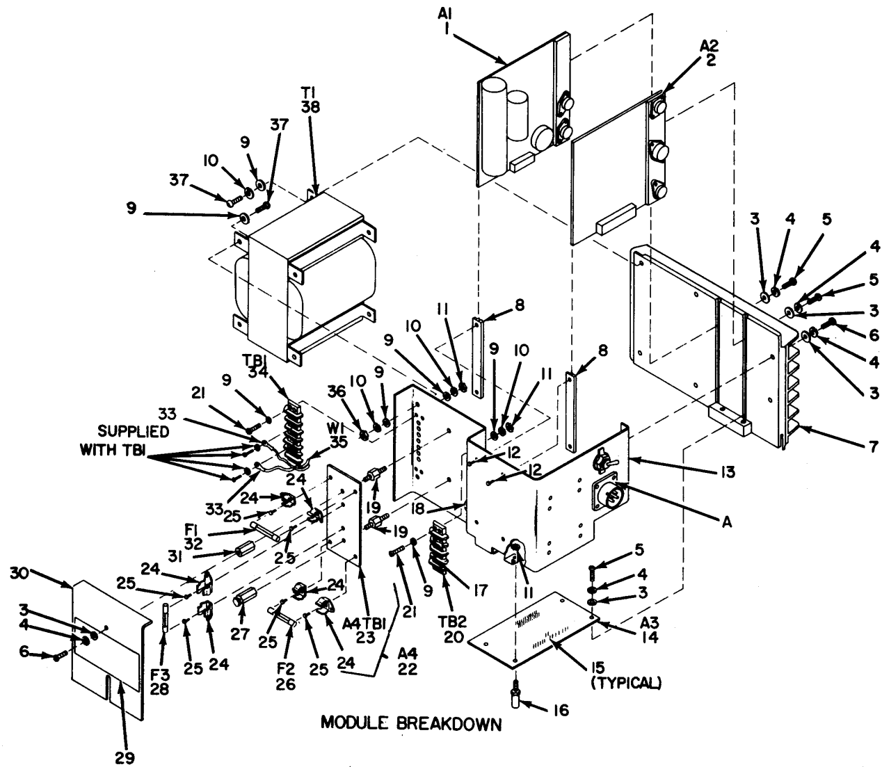
Figure 16. Power Supply Module 6A7 (Sheet 1 of 2).
