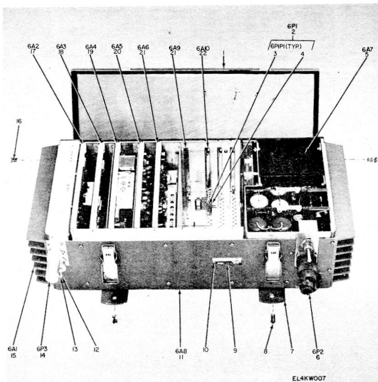
Figure 5. Receiver-Transmitter, Radio RT-1060/URC-80(V)1 and RT-1061/URC-80(V)3.
