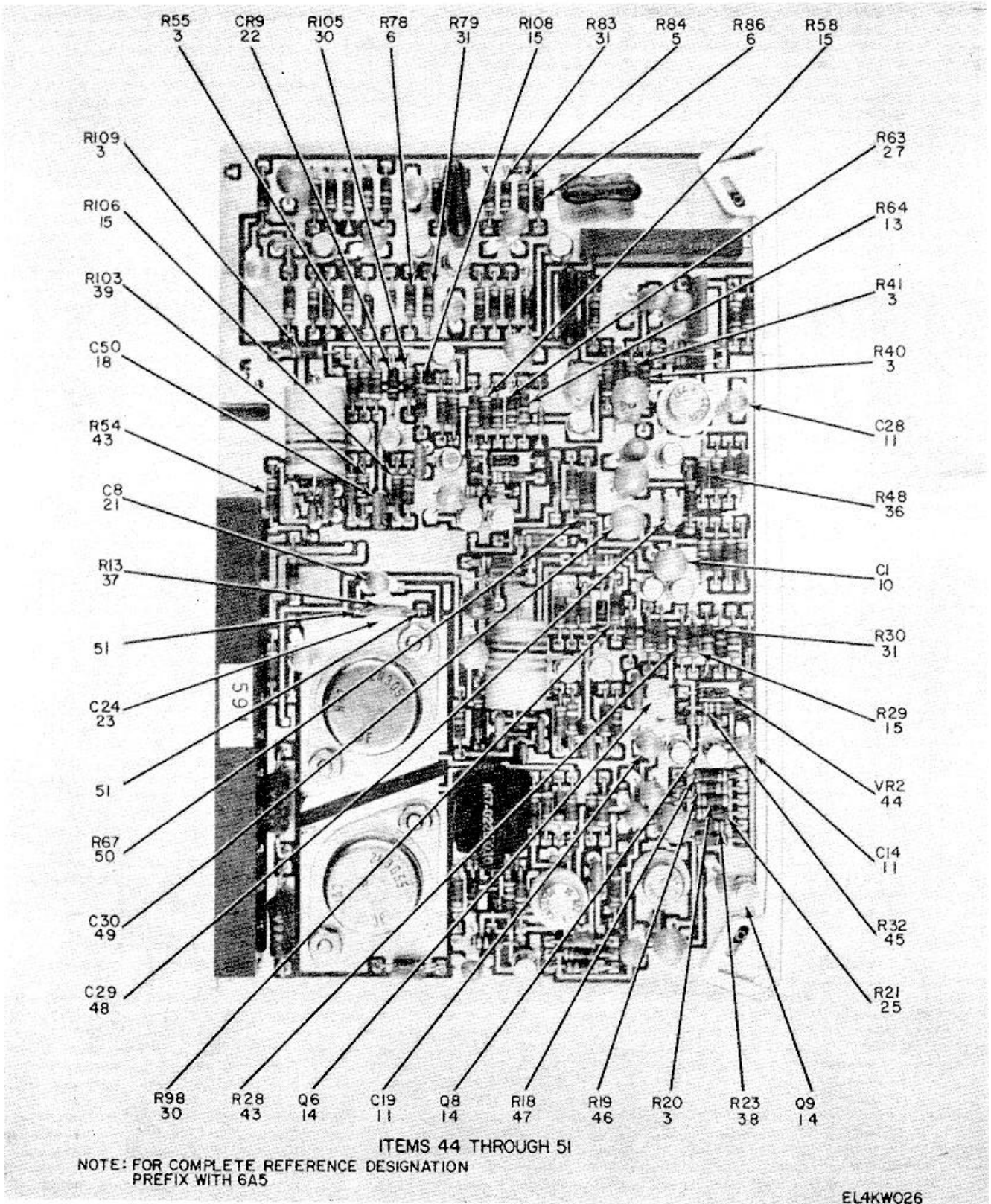
Figure 12. Audio/Squelch Card 6A5 (Sheet 3 of 6).
