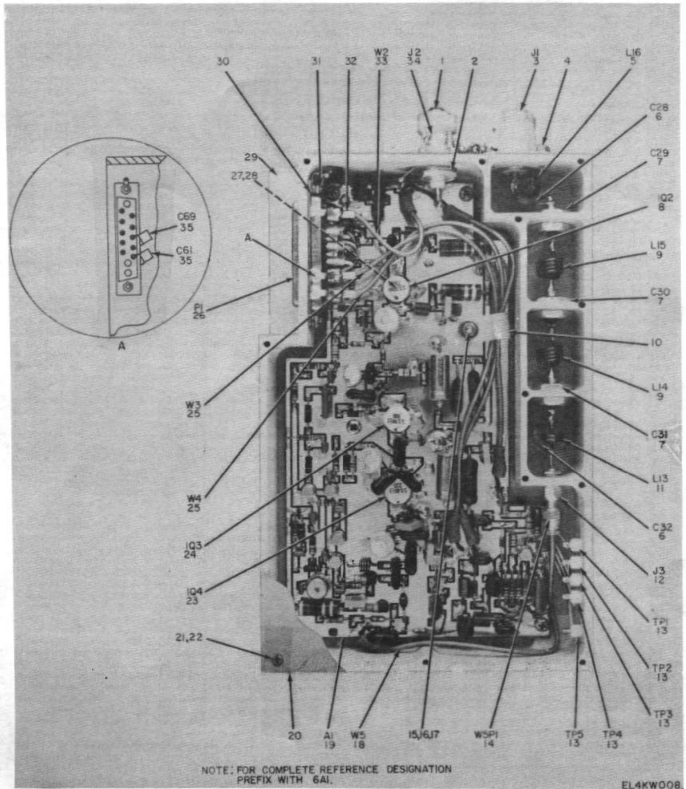
Figure 6. Power Amplifier Module 6A1.
