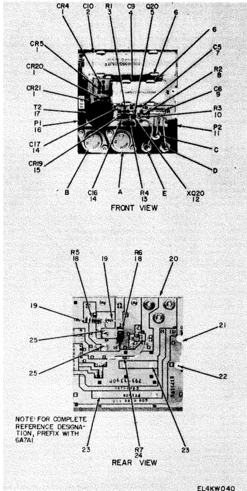
Figure 17. Inverter Card 6A7A1 (Sheet 1 of 3).
