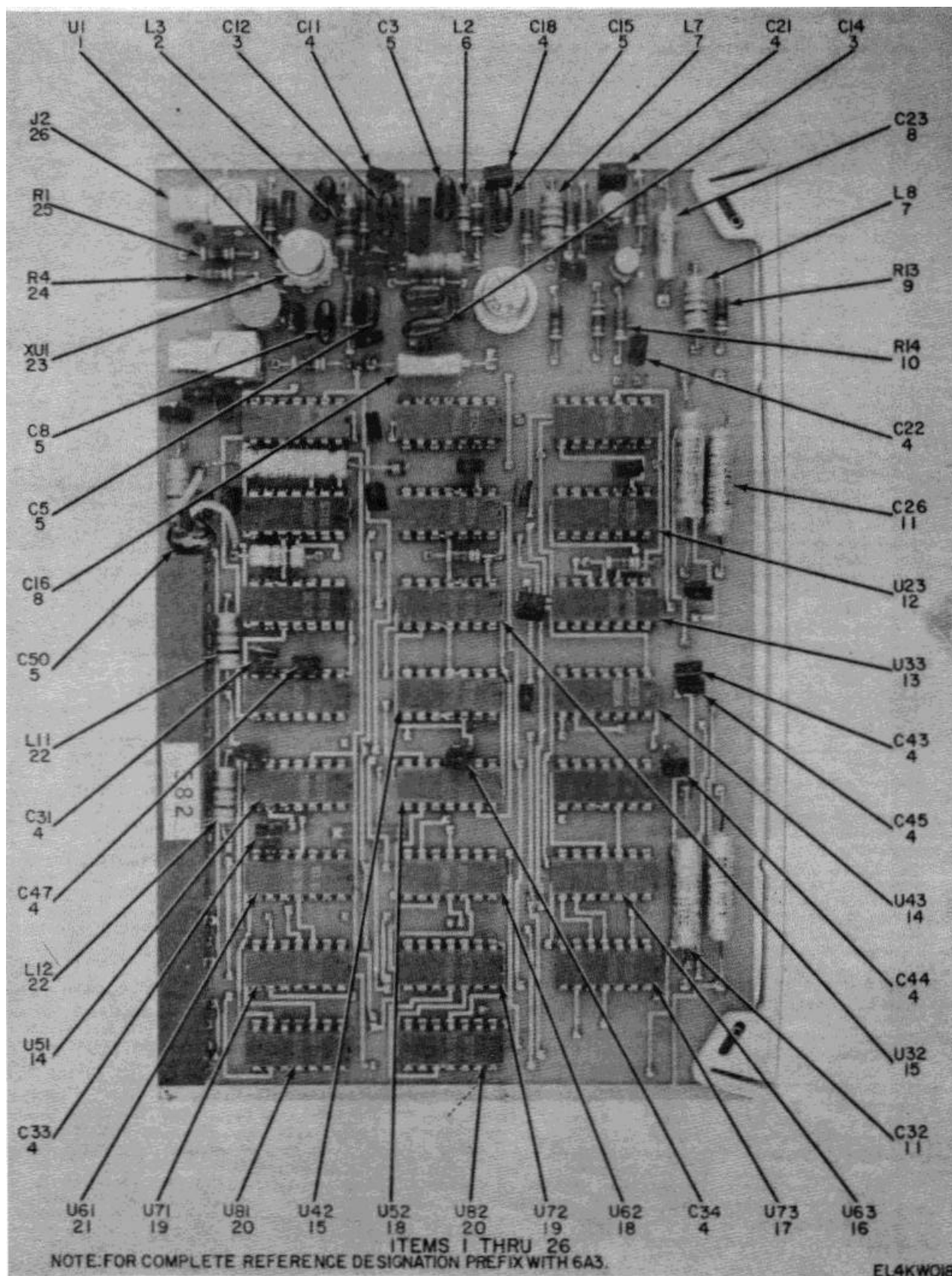
Figure 10. - Mixer/Variable Divider Card 6A3 (Sheet 1 of 3).
