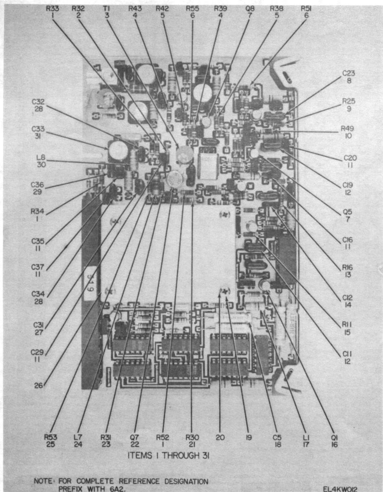
Figure 8. TCXO/Multiplier Card 6A2 (Sheet 1 of 5).
