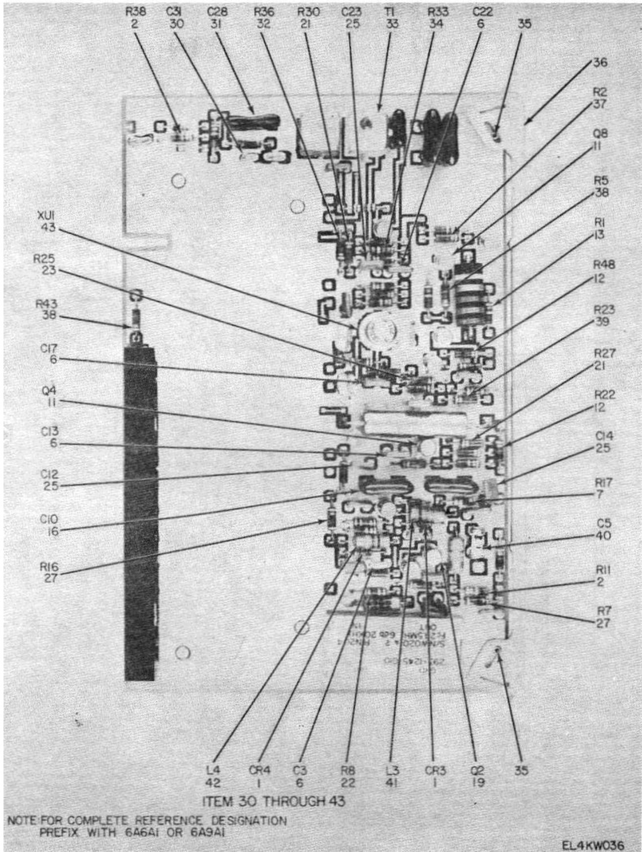
Figure 15. Printed Circuit Board 6A6A1 (Sheet 2 of 3).
