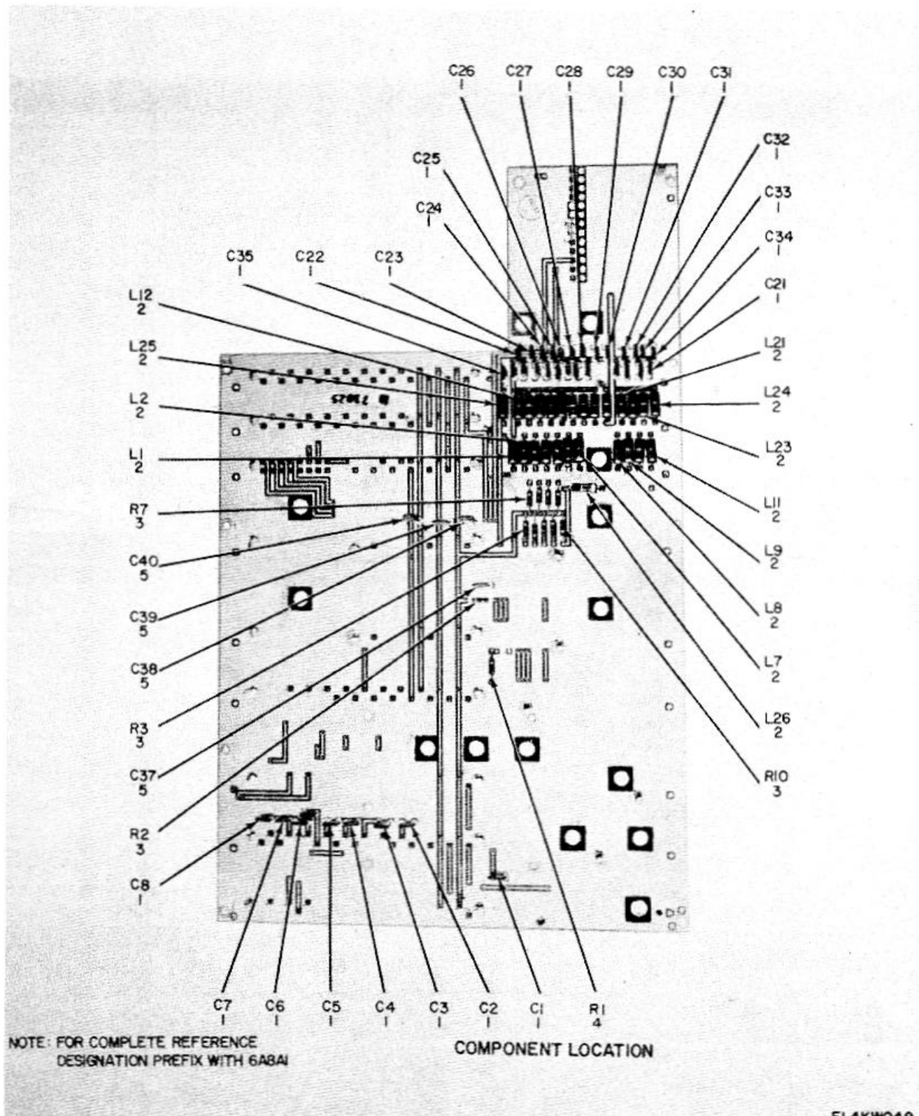
Figure 20. Backplane Board 6A8A1 (Sheet 1 of 3).
