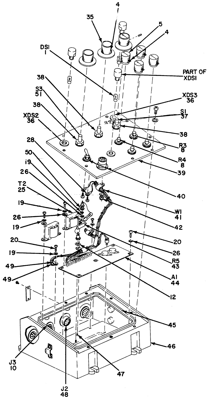
INTERIOR VIEW ADDITIONAL COMPONENT LOCATION NOTE: FOR COMPLETE REFERENCE DESIGNATION PREFIX WITH 2
