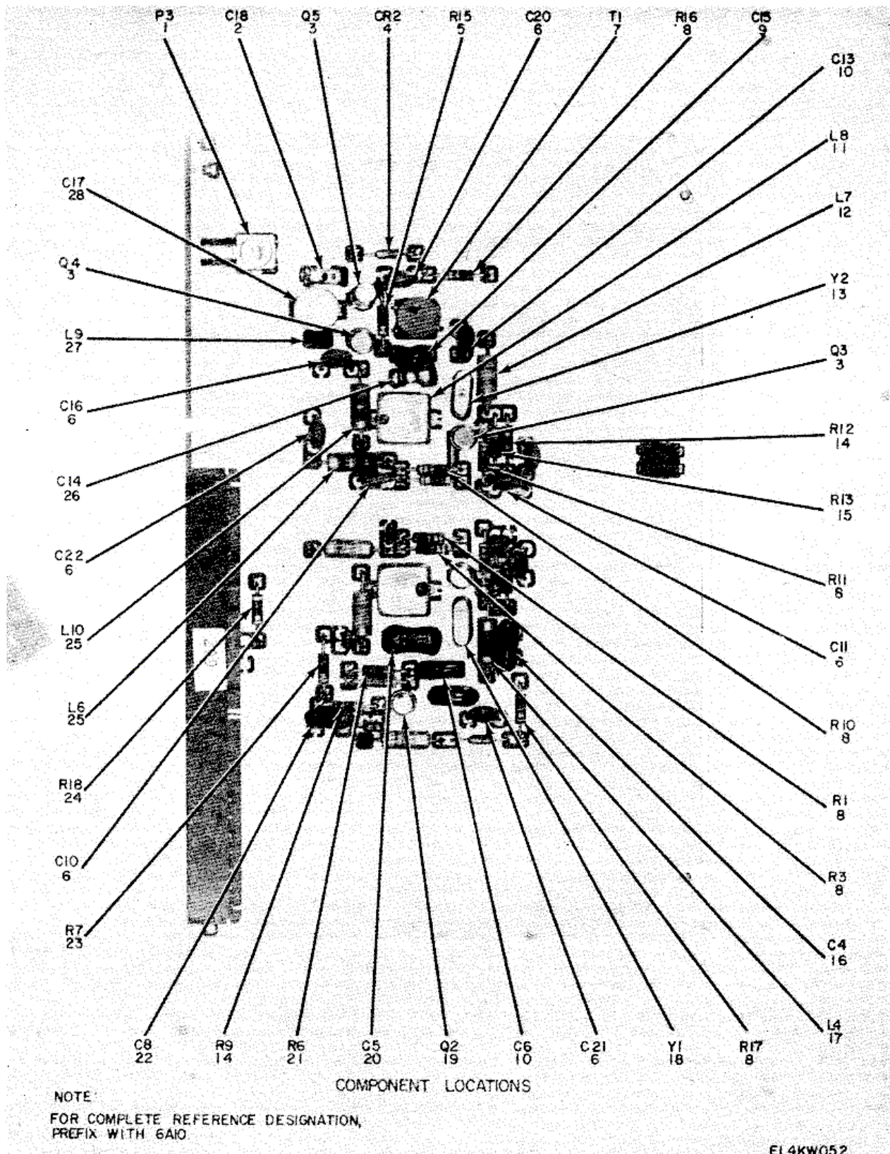
Figure 21. Injection Oscillator Card 6A10 (Sheet 1 of 2).
