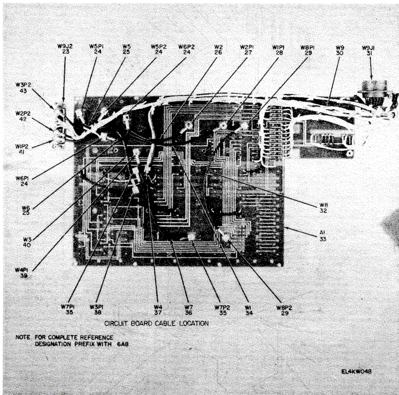
Figure 19. Wired Chassis 6A8 (Sheet 2 of 2).
