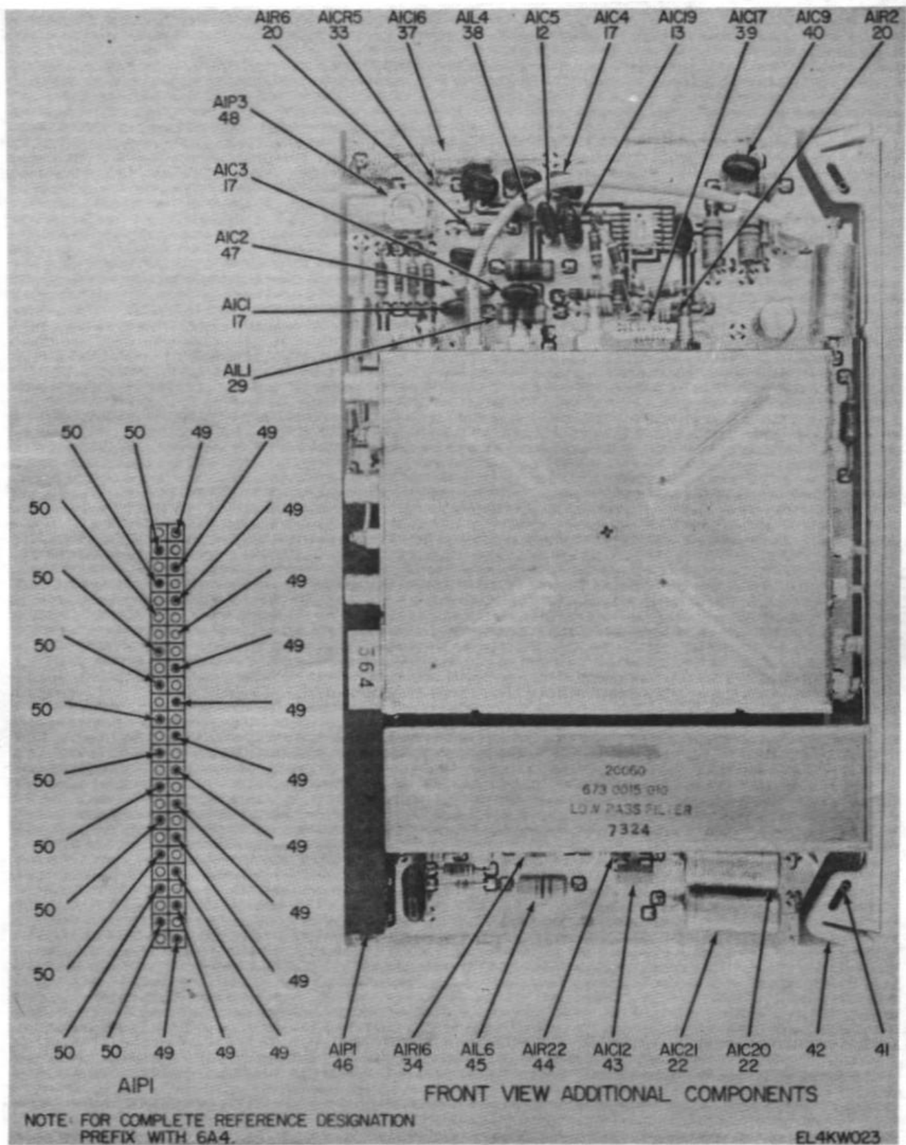
Figure 11. Modulator/VCO Card 6A4 (Sheet 3 of 3).
