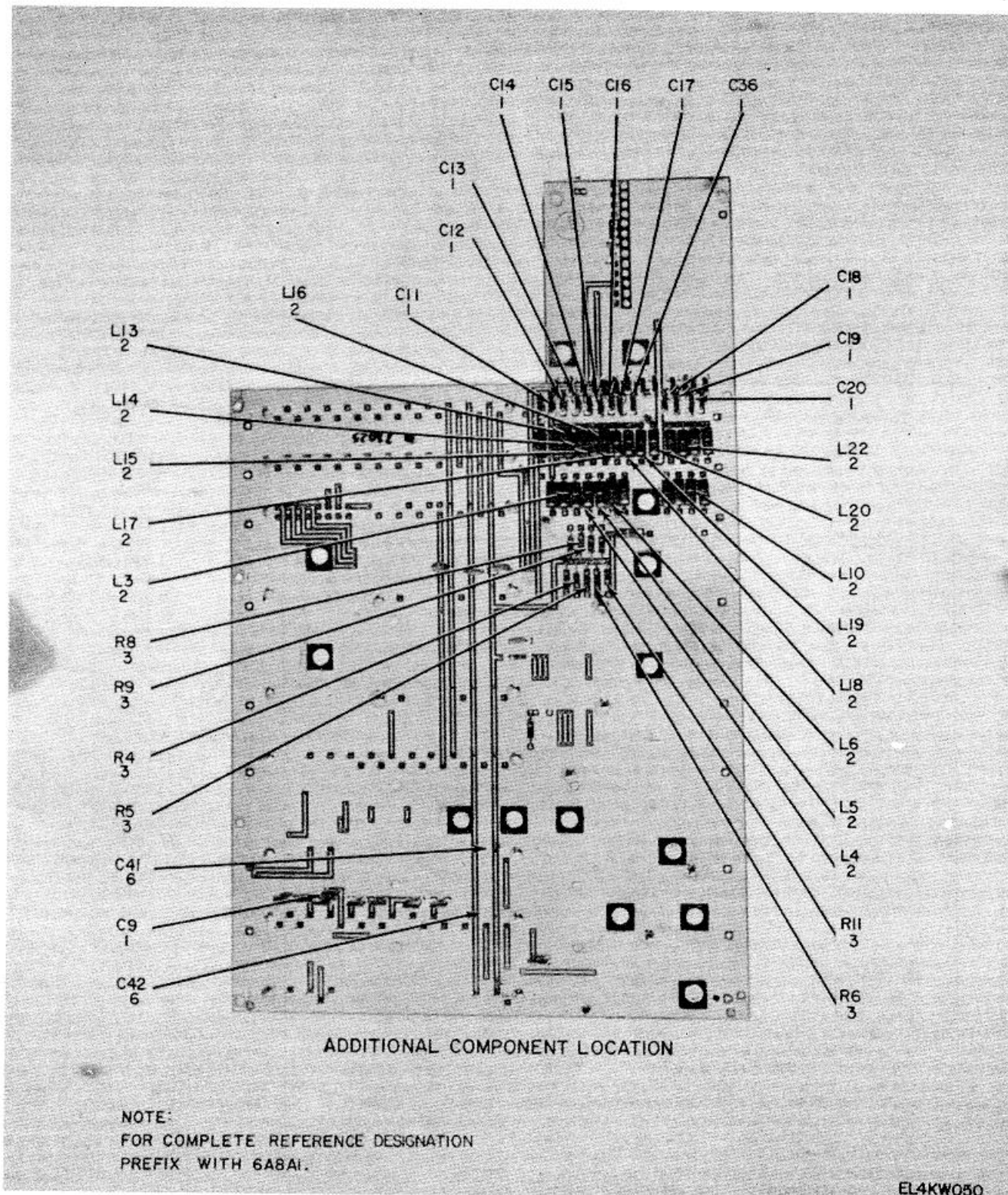
Figure 20. Backplane Board 6A8A1 (Sheet 2 of 3).
