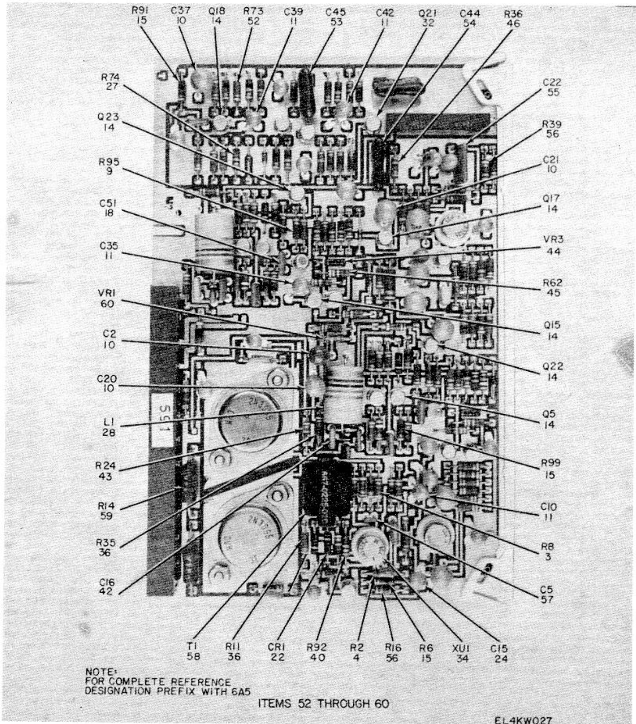
Figure 12. Audio/Squelch Card 6A5 (Sheet 4 of 6).
