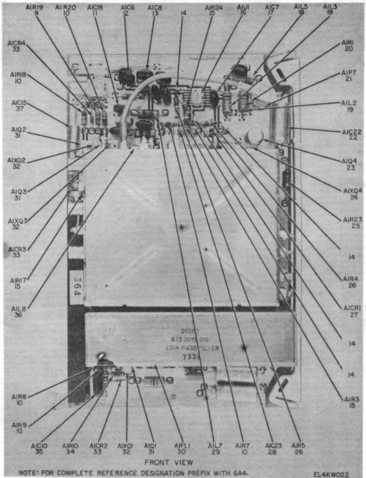
Figure 11. Modulator/VCO Card 6A4 (Sheet 2 of 3).
