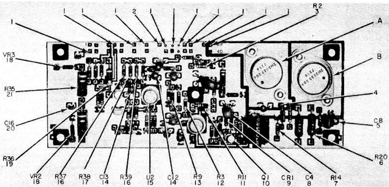
ITEMS 1 THROUGH 21
