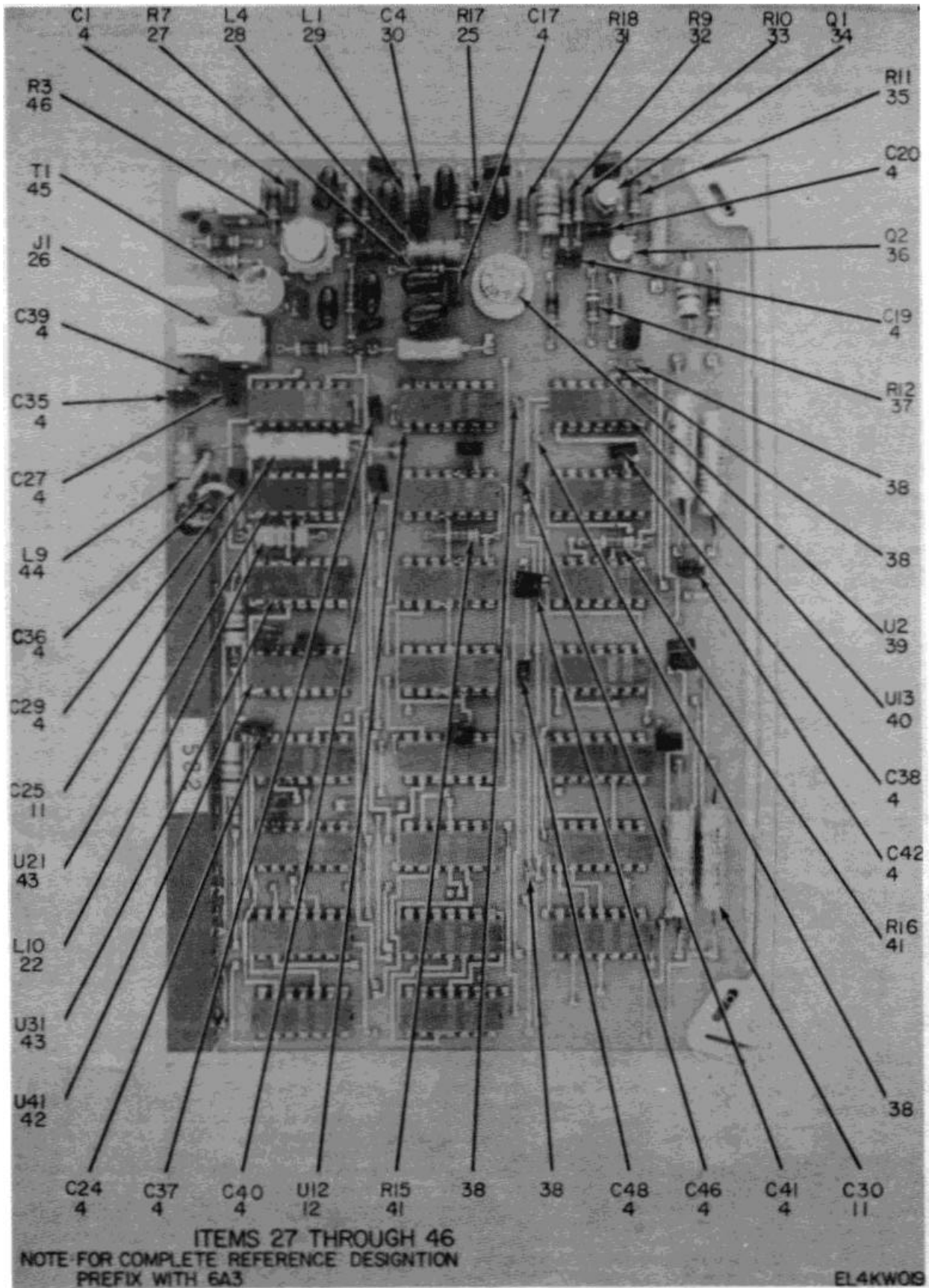
Figure 10. Mixer/Variable Divider Card 6A3 (Sheet 2 of 3).
