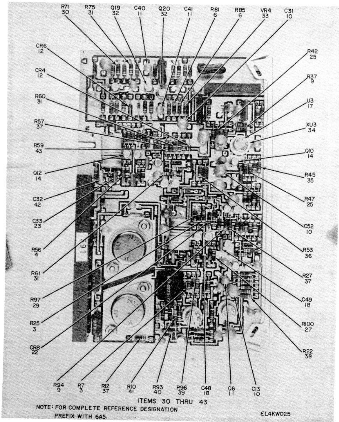
Figure 12. Audio/Squelch Card 6A5 (Sheet 2 of 6).
