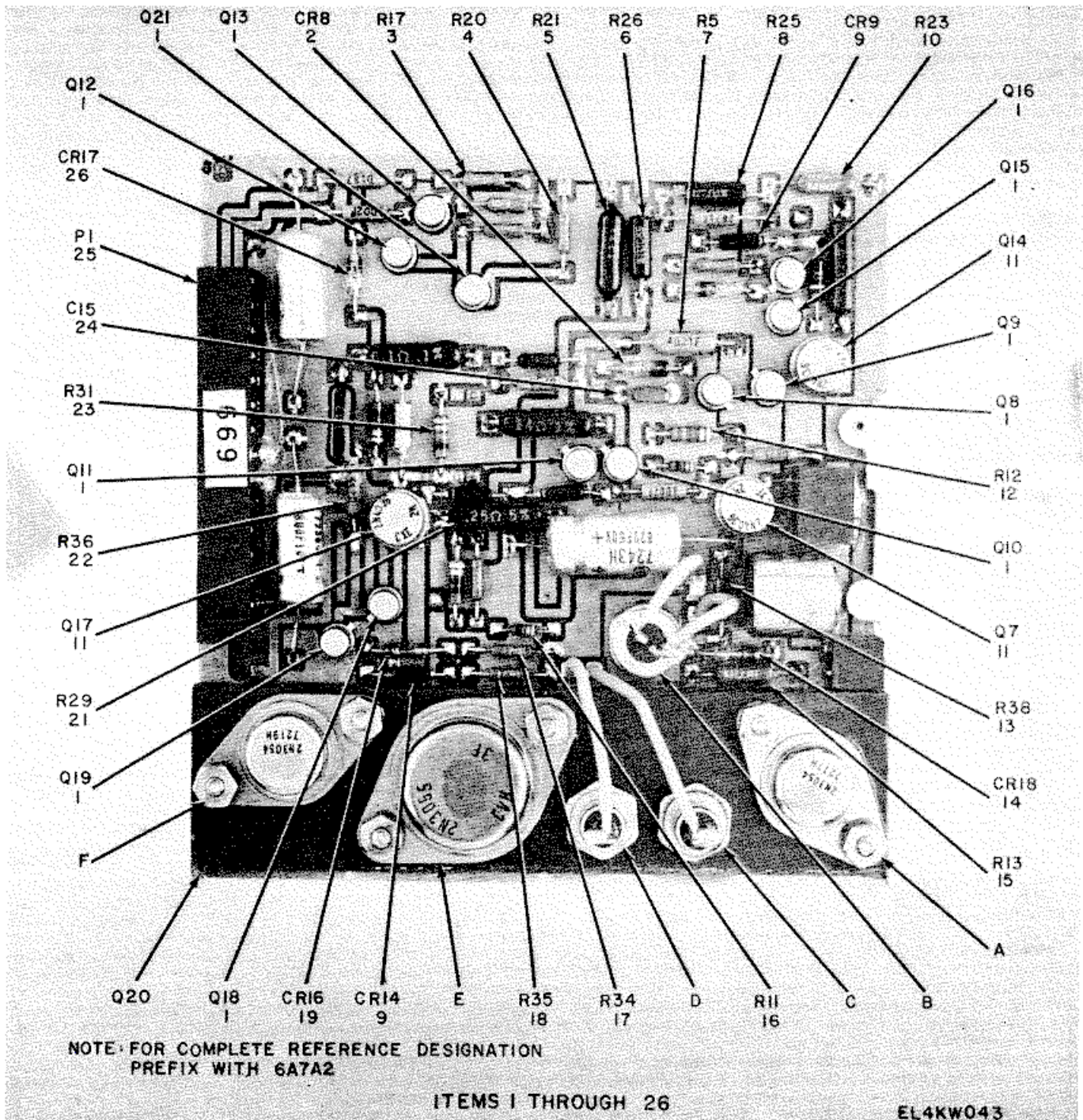
Figure 18. Regulator Card 6A7A2 (Sheet 1 of 4).
