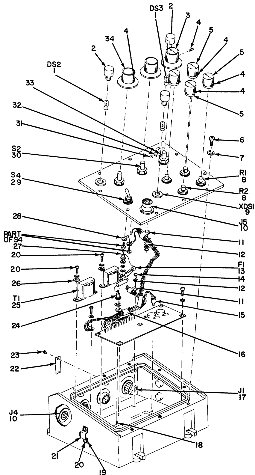
INTERIOR VIEW COMPONENT LOCATION NOTE: FOR COMPLETE REFERENCE DESIGNATION PREFIX WITH 2
