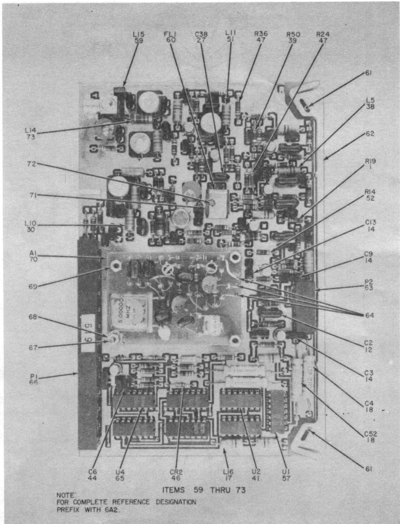
Figure 8. TCXO/Multiplier Card 6A2 (Sheet 4 of 5).
