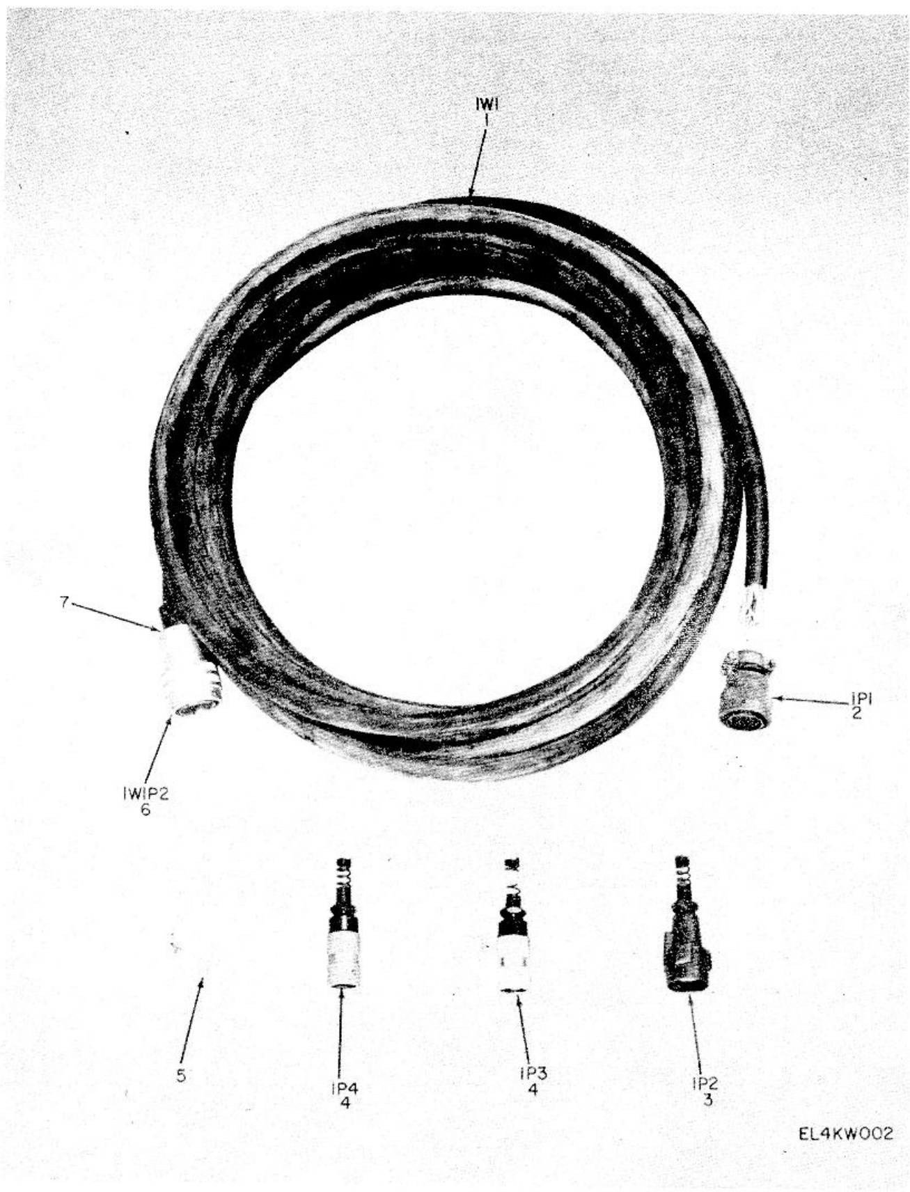
Figure 2. Cable Assembly Kit.
