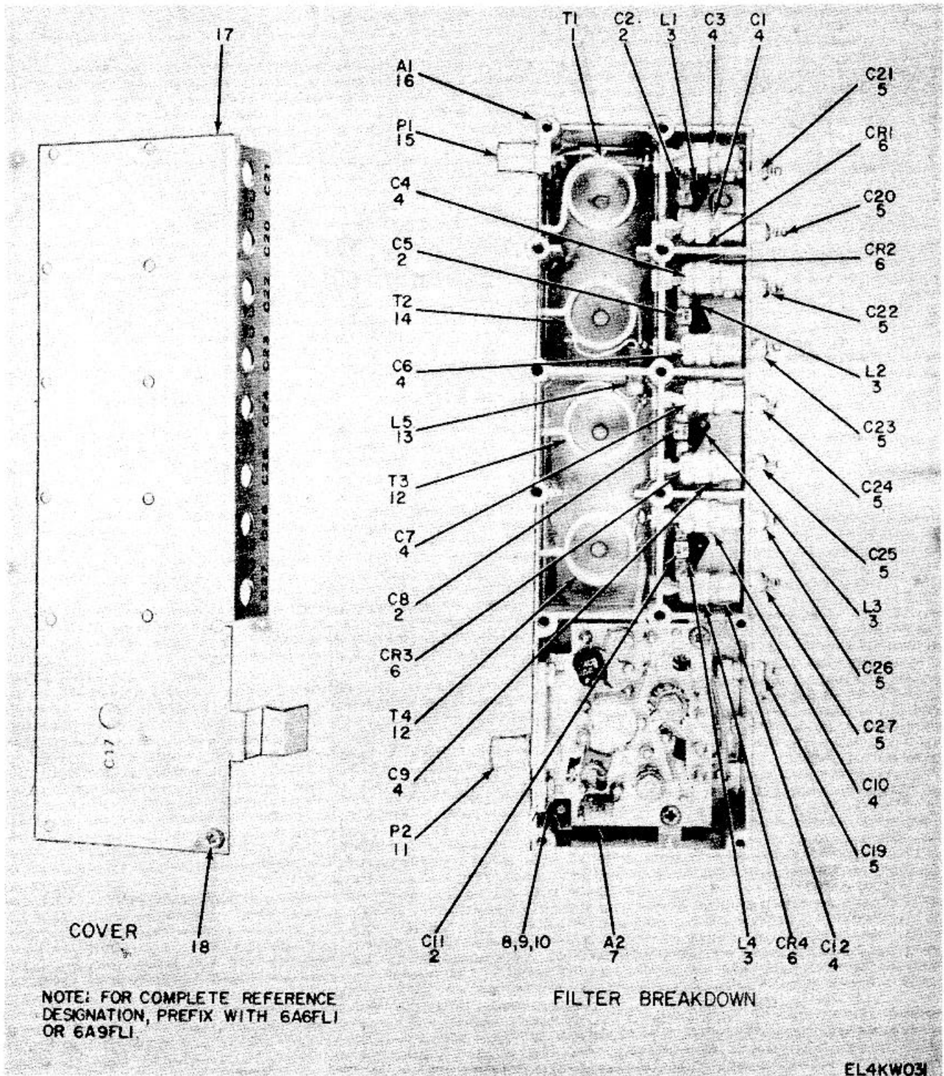
Figure 14. Receiver Filter 6A6FL1 (Sheet 1 of 4).
