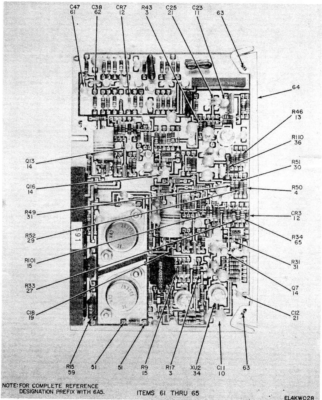
Figure 12. Audio/Squelch Card 6A5 (Sheet 5 of 6).
