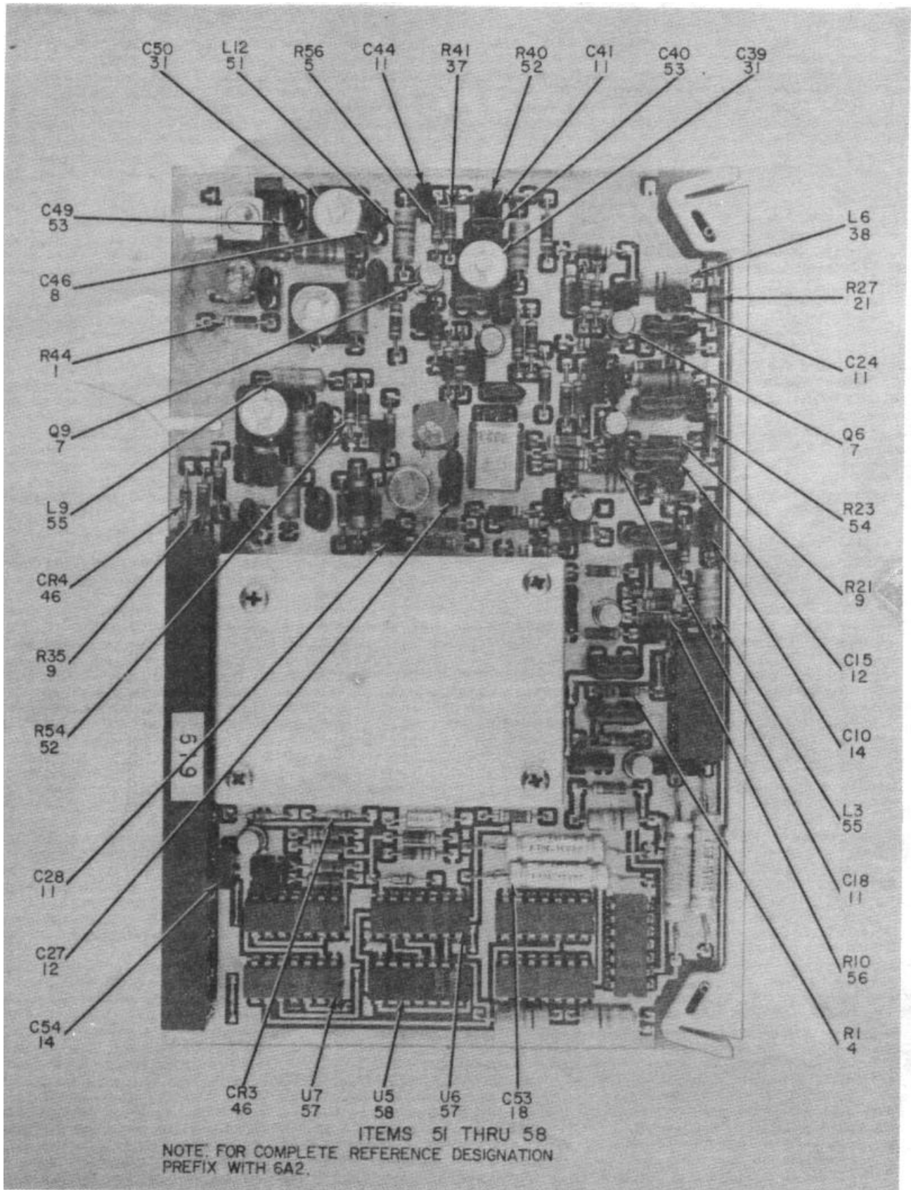
Figure 8. TCXO/Multiplier Card 6A2 (Sheet 3 of 5).
