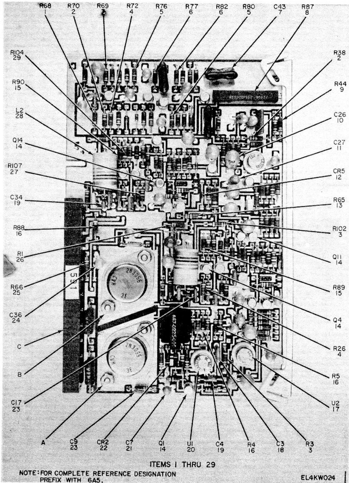
Figure 12. Audio/Squelch Card 6A5 (Sheet 1 of 6).
