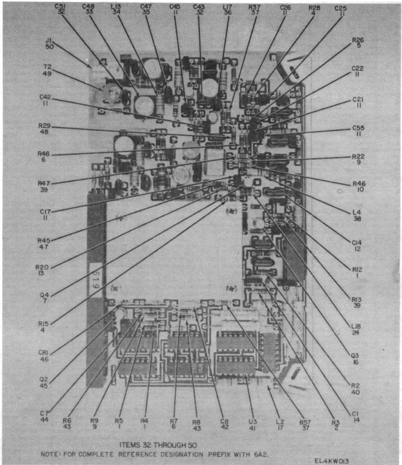
Figure 8. TCXO/Multiplier Card 6A2 (Sheet 2 of 5).
