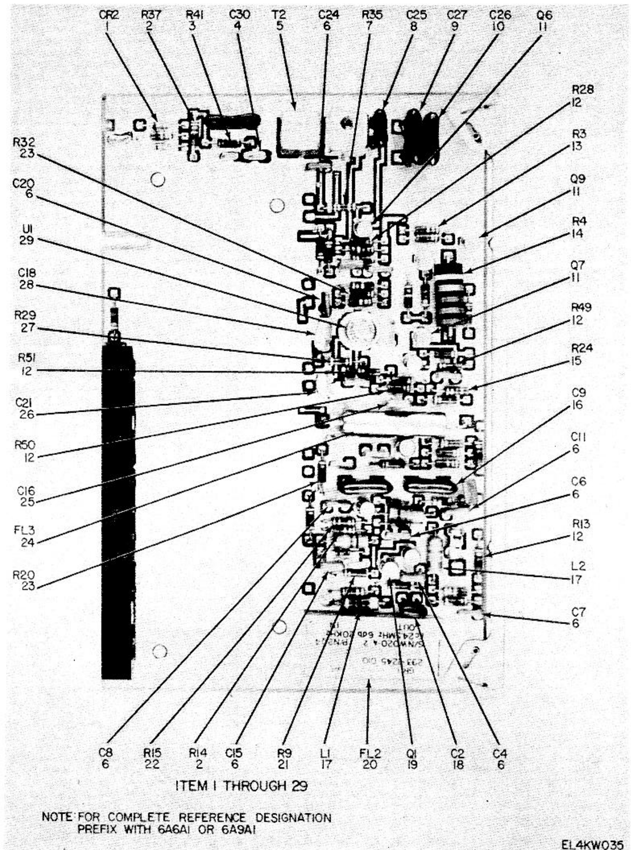
Figure 15. Printed Circuit Board 6A6A1 (Sheet 1 of 3).
